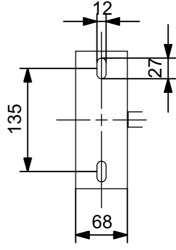
DETAIL A SCALE 1:5
